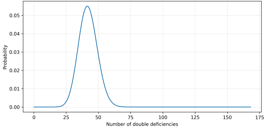
Figure 8: Probability distribution of the number of double deficiencies in \text{Av}_{170}(321, 231) .
