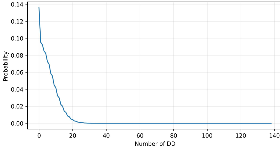
Figure 4: Probability distribution of the number of double deficiencies in \text{Av}_{140}(132) .
