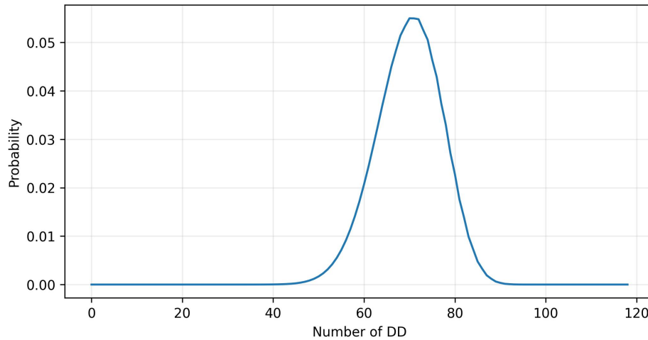
Figure 6: Probability distribution of the number of double deficiencies in \text{Av}_{120}(231) .
