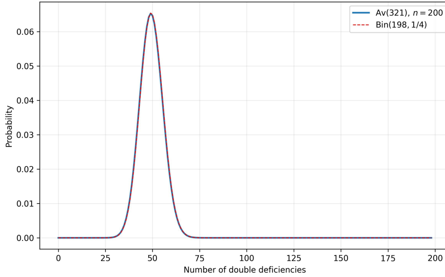
Figure 3: Probability distribution of the number of double deficiencies in \text{Av}_{200}(321) , together with the binomial distribution \text{Bin}(198, \frac{1}{4}) .
