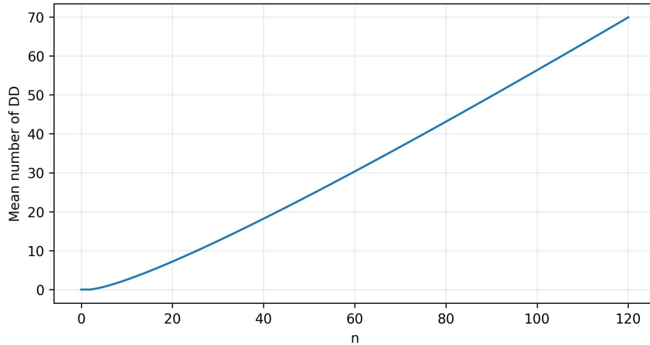
Figure 7: Mean number of double deficiencies in 231-avoiding permutations of length n , for 0 \leq n \leq 120 .
