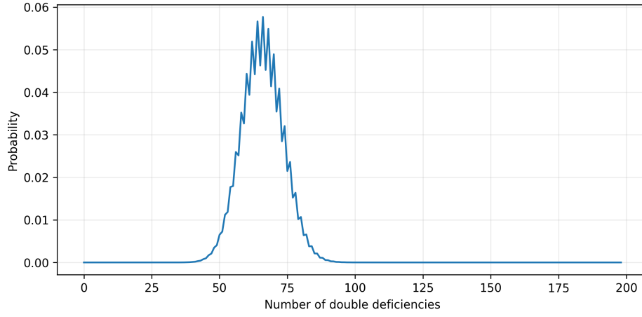
Figure 9: Probability distribution of the number of double deficiencies in \text{Av}_{200}(132, 231) .
