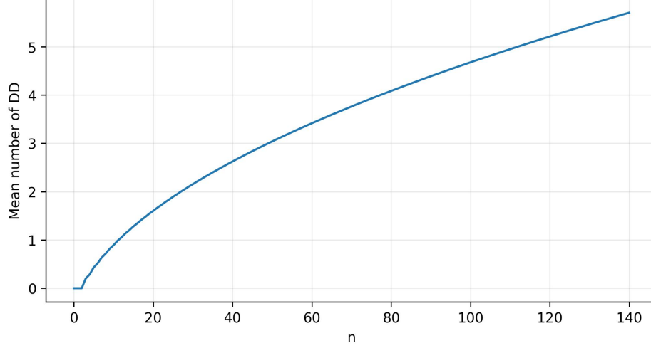
Figure 5: Mean number of double deficiencies in 132-avoiding permutations of length n , for 0 \leq n \leq 140 .
