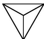
Figure 7: Three compartments of a triangle
