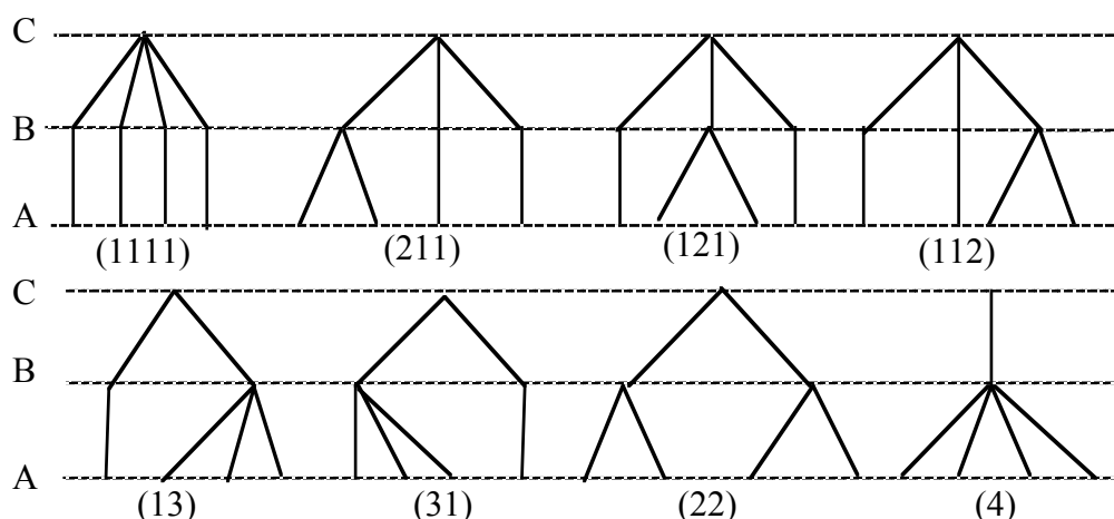
Figure 5: Composition as rooted trees
