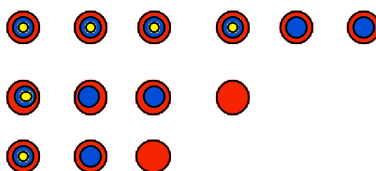
Figure 10: Stacked Ferrers graphs
