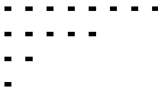
Fig 19: Ferrers' graph of (8521)
