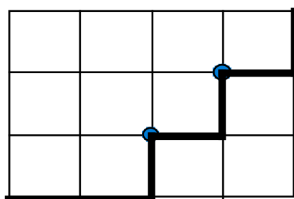
Figure 6: Line of route of a composition
