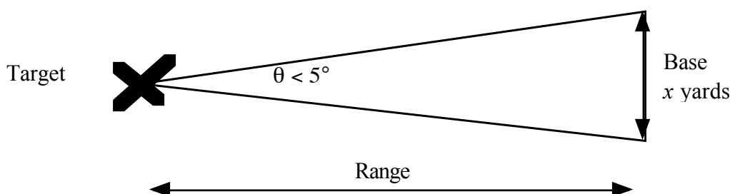
Figure 0: A rule for range finding
