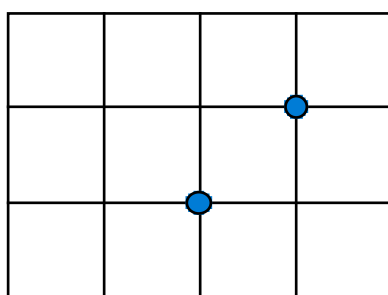
Figure 2: The bipartite number \overline{43}
