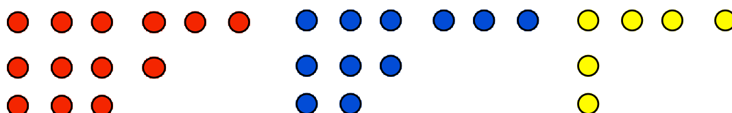
Figure 9: Three Ferrers graph
