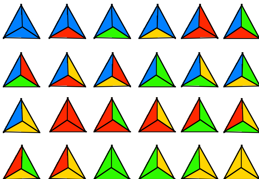
Figure 8: 24 four colour triangles
