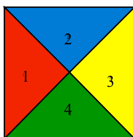
Fig 17: Four colour square
