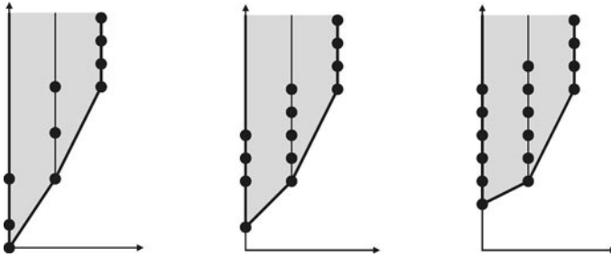
Fig. 7.2 Newton polygons for the example differential equation
