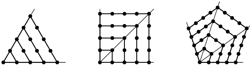
Fig. 3.2 Triangular numbers, square numbers, and pentagonal numbers
