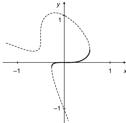
Fig. 6.4 Algebraic curve defining an analytic function in a neighborhood of x = 0
