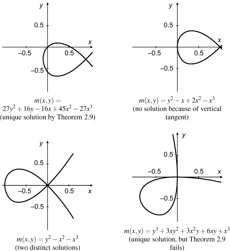
Fig. 6.2 Existence of power series solutions in \mathbb{R}[[x]] for some polynomial equations
