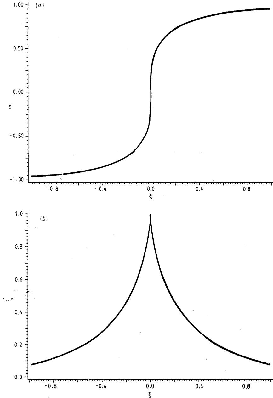
Figure 1. Plots for (a) \varepsilon and (b) 1-r against \xi where \xi = x - x_0 - 4t .
