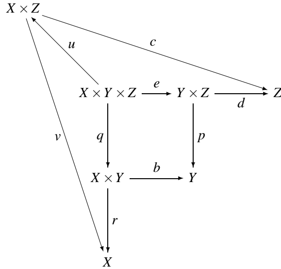
FIGURE 17A.1. Composition of correspondences
