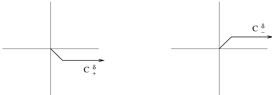
Figure 5: The deformed integration contours C_+^\delta and C_-^\delta .
