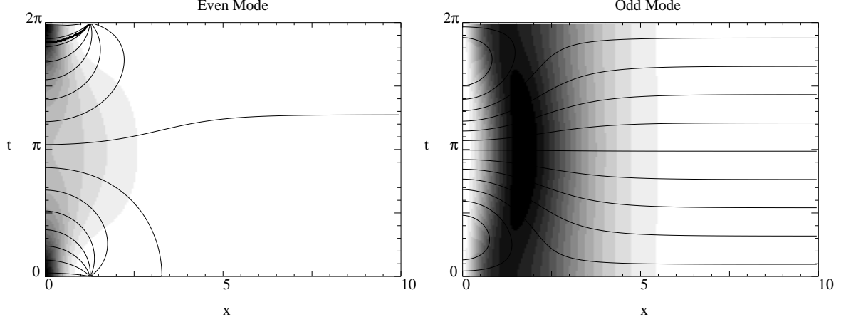
Figure 4: Equal phase contours for the even (left) and odd (right) modes superimposed on a density plot of the corresponding square modulus. The parameter values are \rho_1 = 1/4 and \rho_2 = 3/4 . Here, the Floquet multiplier is not equal to 1, and the modes are not periodic in t , although they have Bloch form.
