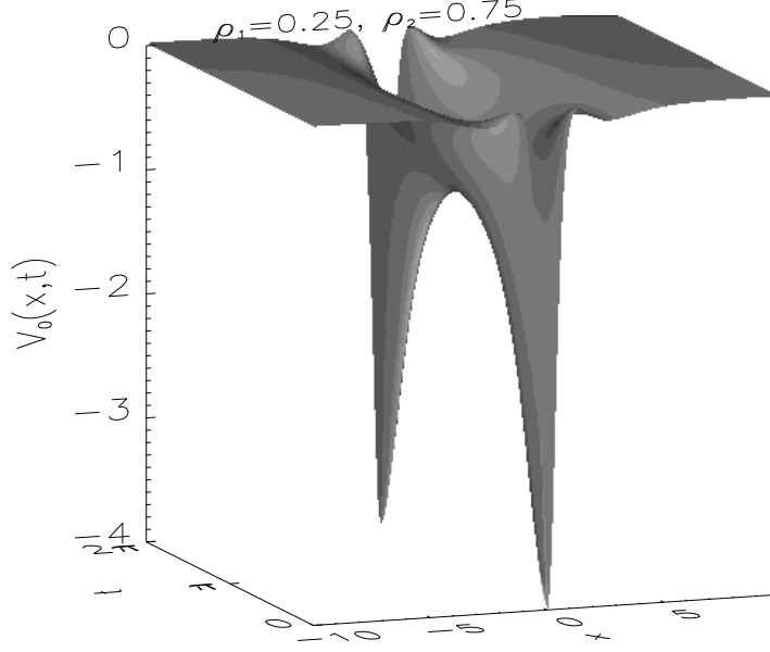
Figure 2: The potential well V_0(x, t) for \rho_1 = 1/4 and \rho_2 = 3/4 . The phase parameters are \theta_1 = \theta_2 = 0 . This well is time-periodic with period L = 2\pi and even in x .
