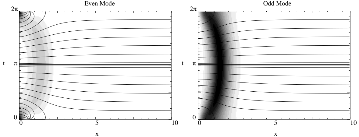
Figure 3: Equal phase contours for the even (left) and odd (right) modes superimposed on a density plot of the corresponding square modulus. The parameter values are \rho_1 = 1/\sqrt{2} and \rho_2 = 1 . For these values of \rho_1 and \rho_2 , the Floquet multiplier is equal to 1, and therefore these are periodic functions of t .
