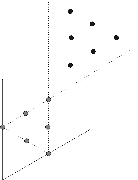
FIGURE 10. \text{Ind}_T^G \chi_{Z_{(\omega_1+\omega_2)/2}^{\text{ss}}}(E)
