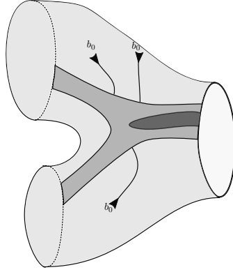
FIGURE 11. Disks defining the homotopy operator
