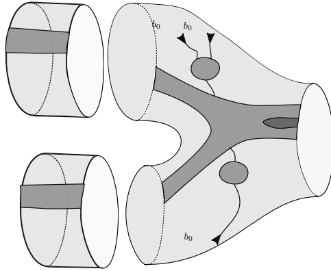
FIGURE 15. Contributions to \delta_+ h(b_0)
