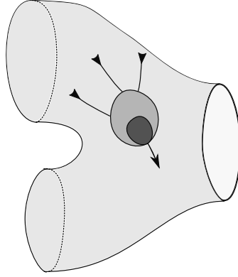
FIGURE 8. A quilted disk in a cobordism
