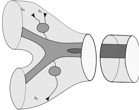
FIGURE 16. Contributions to h(b_0)\delta_-
