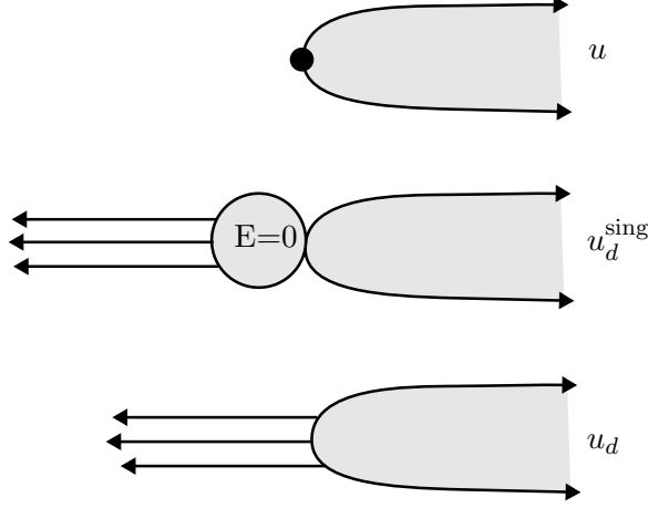
FIGURE 2. Adding multiple trajectories at an intersection point
