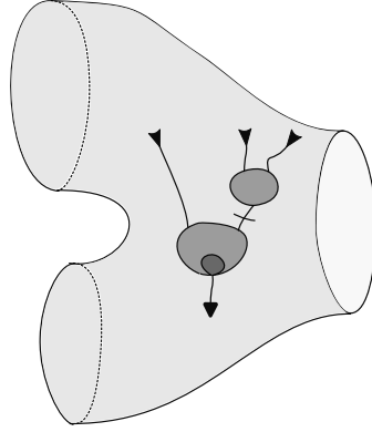
FIGURE 10. Contributions involving m(b_0)
