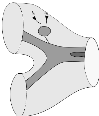
FIGURE 14. Contributions involving m(b_0)
