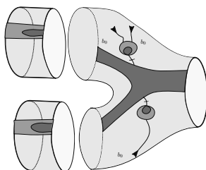
FIGURE 13. Contributions to \varphi(L, b_1)
