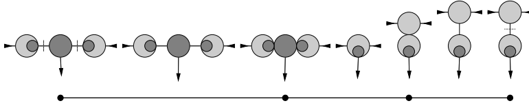
FIGURE 7. Moduli space of treed quilted disks
