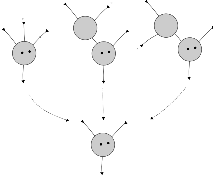
FIGURE 3. Examples of the forgetful map
