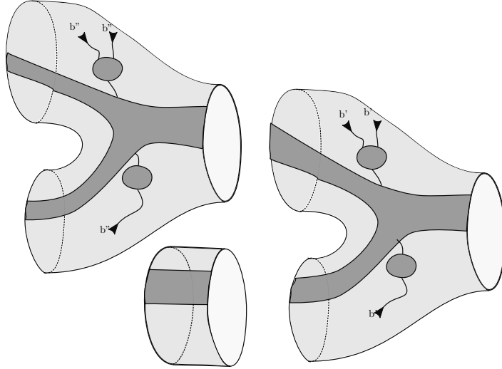
FIGURE 17. Composition of bounding chains
