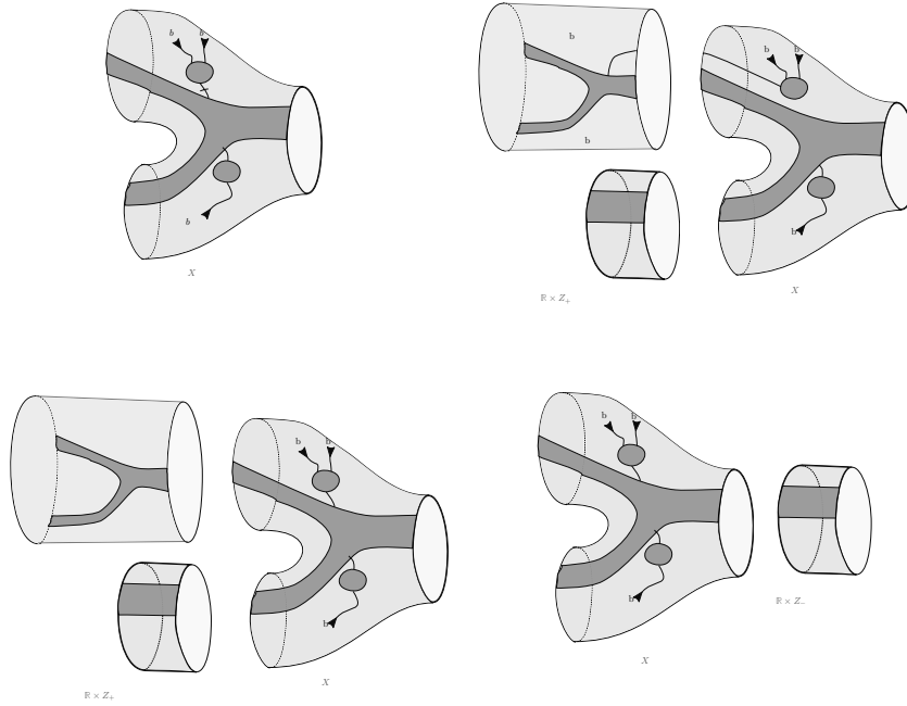
FIGURE 6. Boundaries of moduli spaces bounding the Lagrangian
