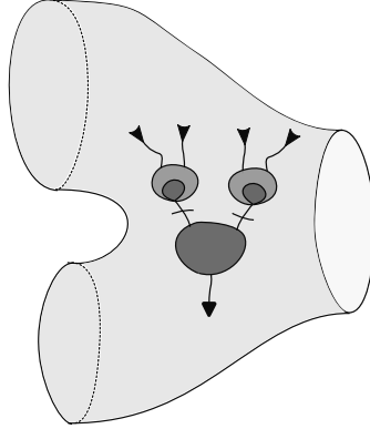
FIGURE 9. Contributions giving m(b_1)
