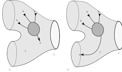
FIGURE 5. Holomorphic curves defining the curvature
