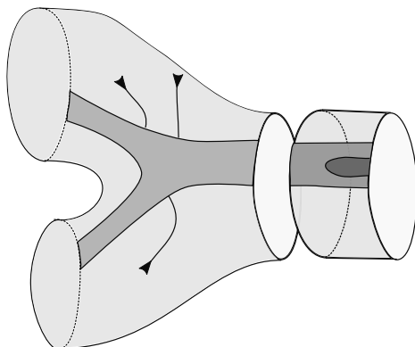
FIGURE 12. Contributions to \varphi(L, b_0)
