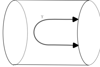
FIGURE 19. A one-dimensional Lagrangian with cylindrical ends
