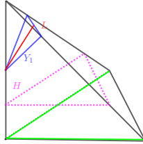
FIGURE 18. Separating the Lagrangian from the rational blow-downs
