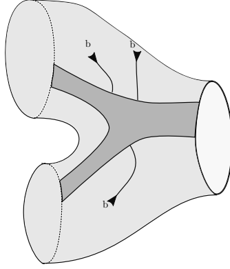
FIGURE 4. Disks defining the chain map
