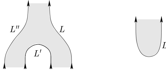
FIGURE 1. Composition and identity in the Donaldson-Fukaya category
