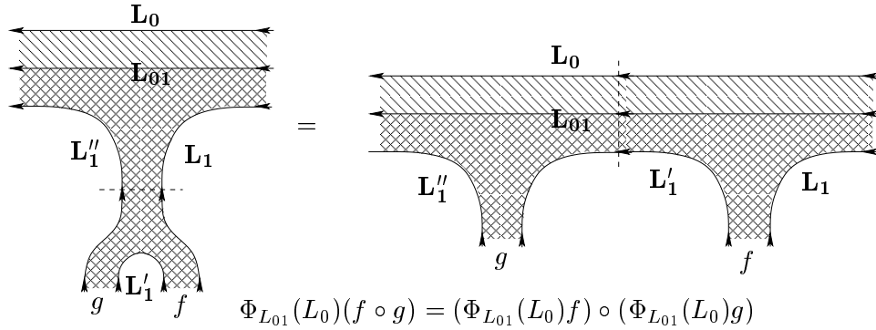
FIGURE 5. Composition axiom for Lagrangian functors
