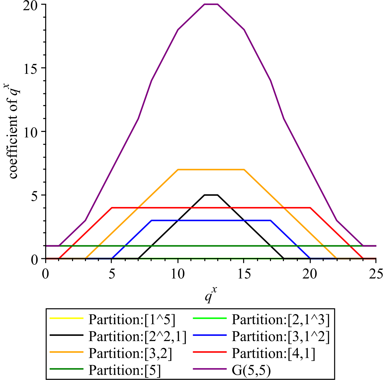
Figure 1: Contributions from Different Partitions to Produce G(5,5) .
