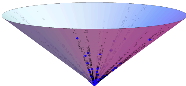
FIGURE 2. A piece of the thin Pythagorean orbit \mathcal{O} in (3.28). Points \mathbf{x} \in \mathcal{O} are again marked according to whether the “area” f(\mathbf{x}) = \frac{1}{12}xy is in \mathcal{P}_R with R \leq 3 (●), R = 4 (●), or R \geq 5 (●).
