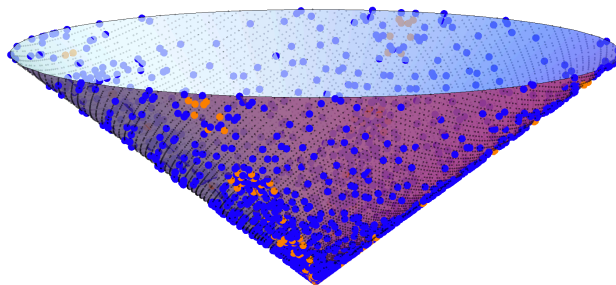
FIGURE 1. A piece of the cone V in (3.9) with markings at the primitive Pythagorean triples \mathbf{x} . Points \mathbf{x} are marked according to whether the “area” f(\mathbf{x}) = \frac{1}{12}xy is in \mathcal{P}_R with R \leq 3 (●), R = 4 (●), or R \geq 5 (●).
