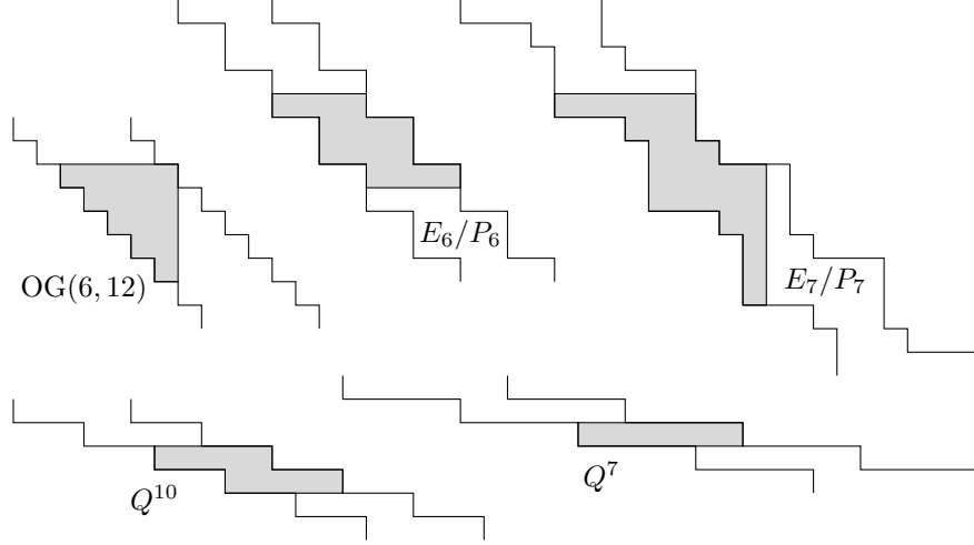
FIGURE 1. The partially ordered sets \widehat{\mathcal{P}}_X for a collection of cominuscul flag varieties, with the boxes of \mathcal{P}_X colored gray.
