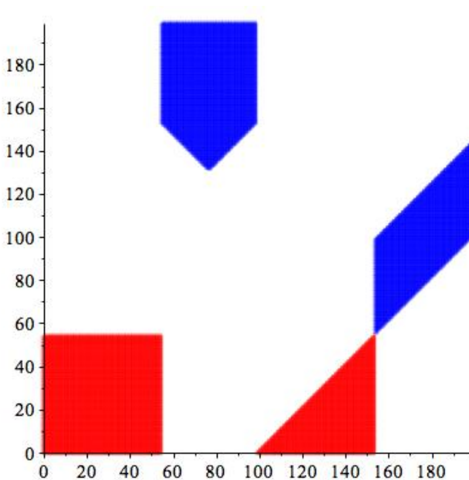
Figure 8: The Nearly Optimal One Square and One Triangle (with the same side length) Configuration for a 200 by 200 Chess Board
