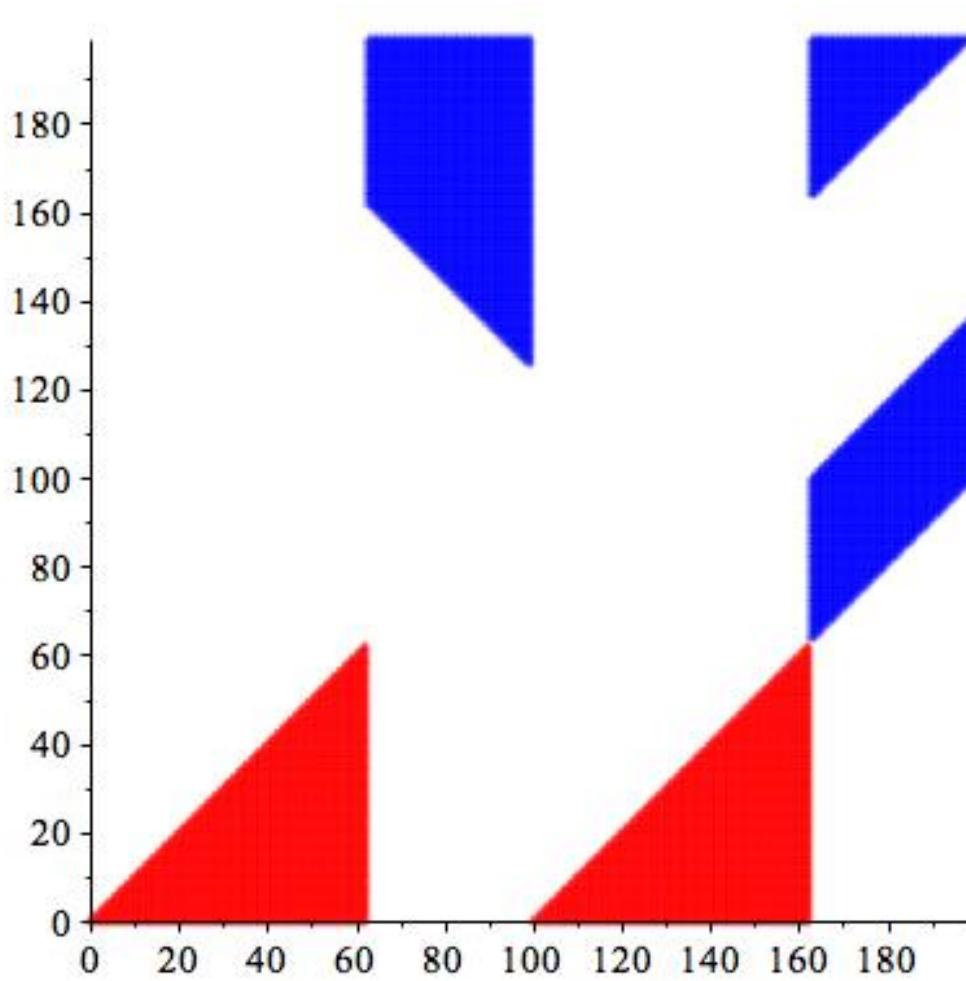
Figure 7: The Nearly Optimal Two Identical Triangles Isosceles Right Configuration for a 200 by 200 Chess Board
