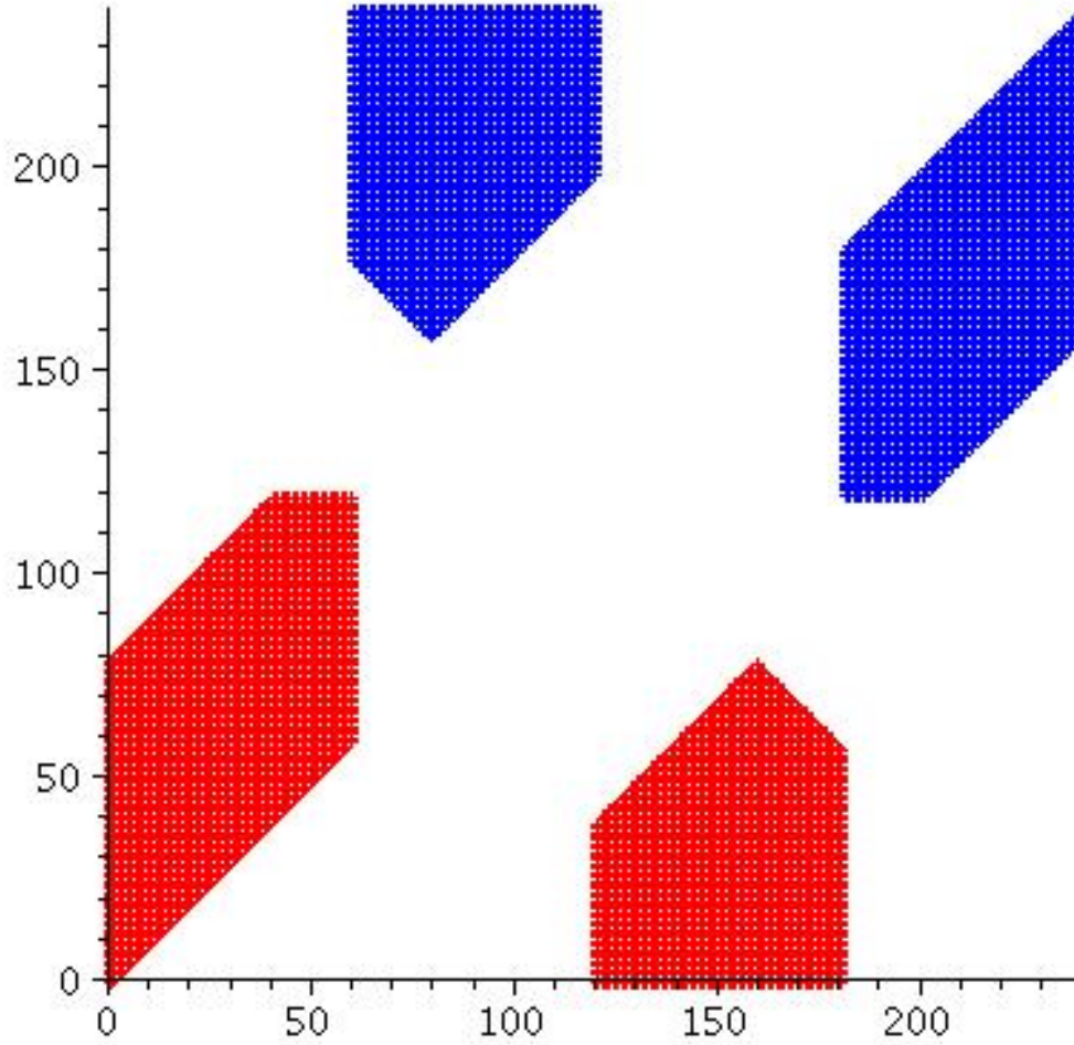
Figure 1: The Benoit Jubin's Construction for a 240 by 240 Chess Board
