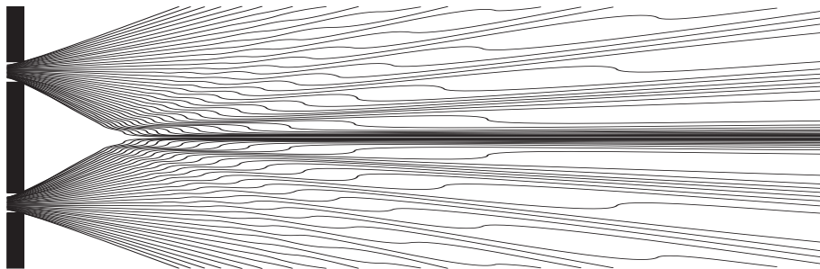
Figure 1: An ensemble of trajectories for the two-slit experiment, uniform in the slits. (Drawn by G. Bauer from [9].)
