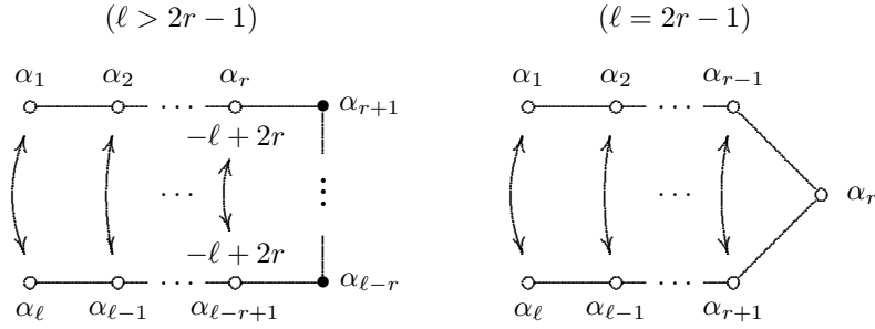
FIGURE 15. Marked Satake diagrams for \mathbf{SL}_{\ell+1}/\mathbf{S}(\mathbf{GL}_r \times \mathbf{GL}_{\ell+1-r})
