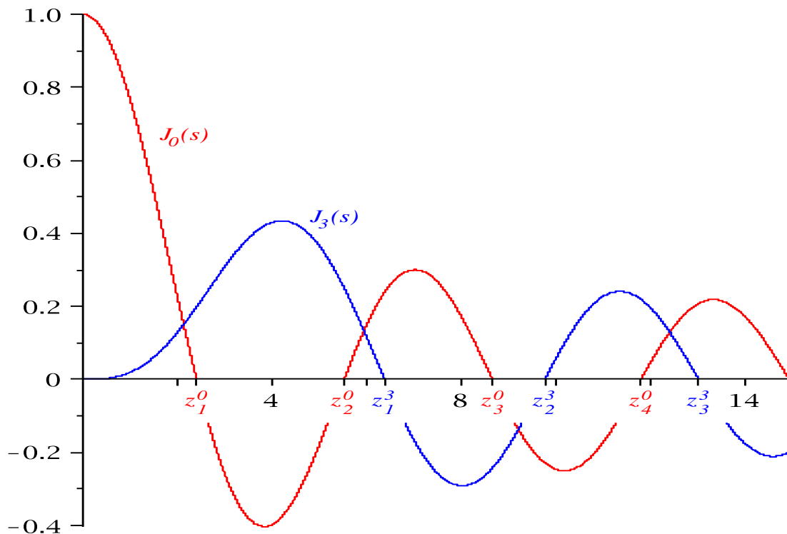
Figure 1. The Bessel functions J_0(s) and J_3(s) for s \geq 0 . The first four zeros of J_0(s) are marked as z_1^0 , z_2^0 , z_3^0 , and z_4^0 , and the first three zeros of J_3(s) as z_1^3 , z_2^3 , and z_3^3 .
