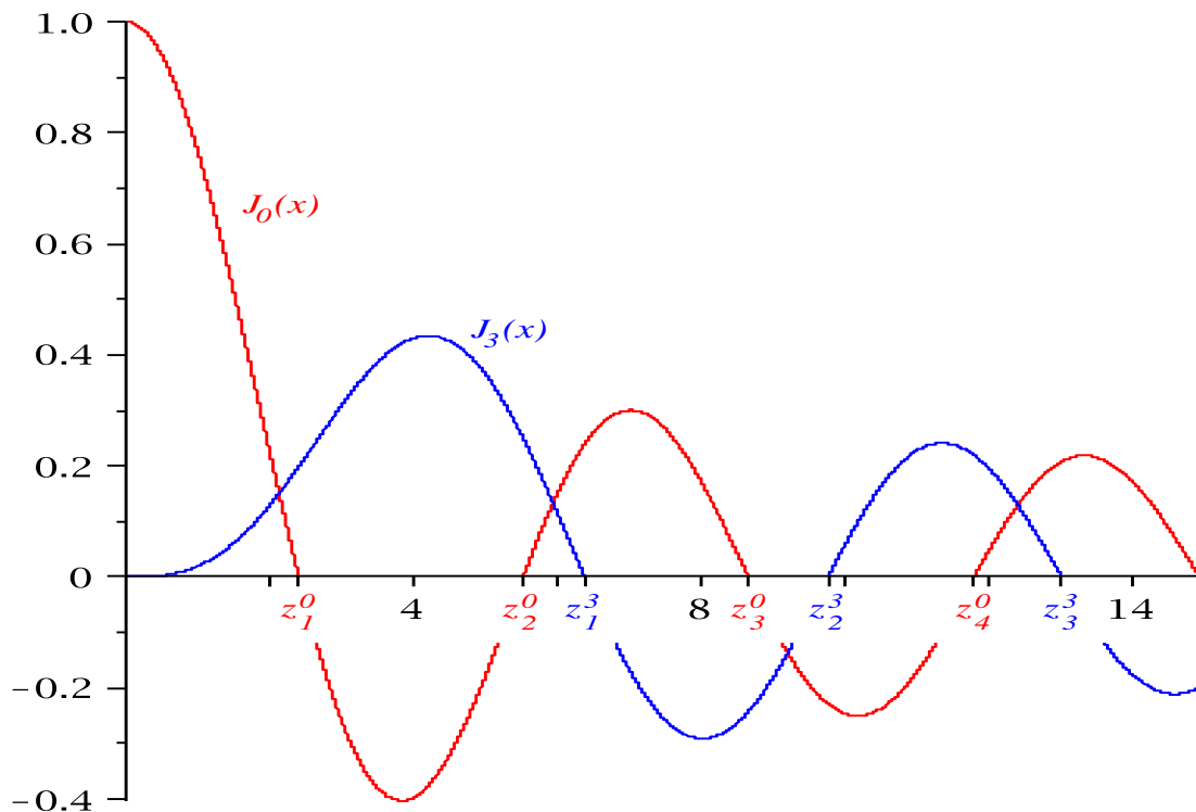
Figure 1. The Bessel functions J_0(x) and J_3(x) for x \geq 0 . The first four zeros of J_0(x) are marked as z_1^0 , z_2^0 , z_3^0 , and z_4^0 , and the first three zeros of J_3(x) as z_1^3 , z_2^3 , and z_3^3 .
